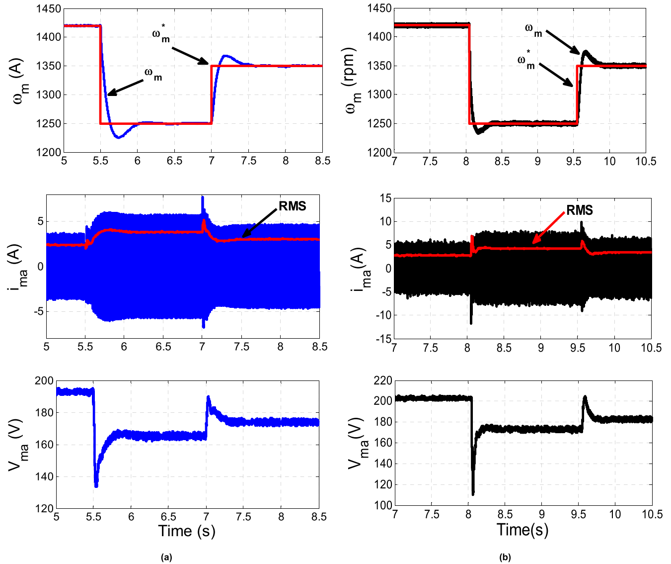
FIGURE 11. Variation of the motor speed, current and phase voltage at step change in the reference speed. (a) Simulation. (b) Experimental.
